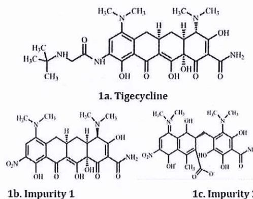
Fig. 1: Molecular structure of tigecycline and its impurities in the study
