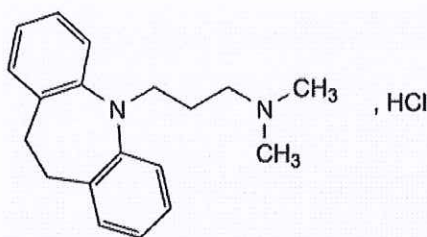
Fig: 1 Structure of Imipramine HCL
