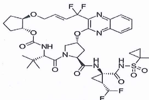
Fig.2. Chemical structure: Glecaprevir
